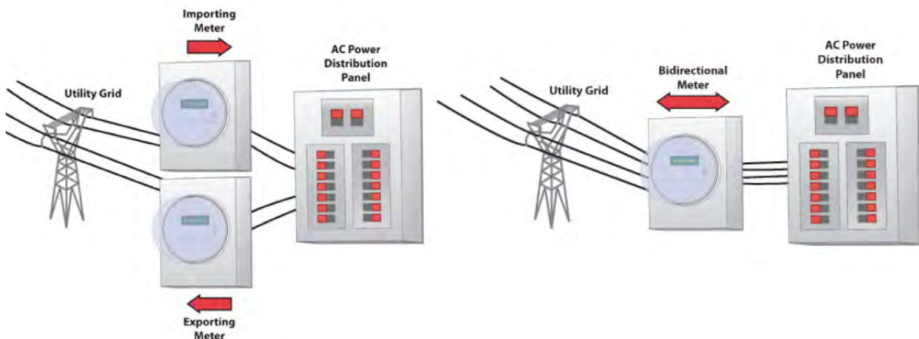
Figure 4: Dual and Bi-Directional Metering Configurations for Grid-Tied Solar PV
